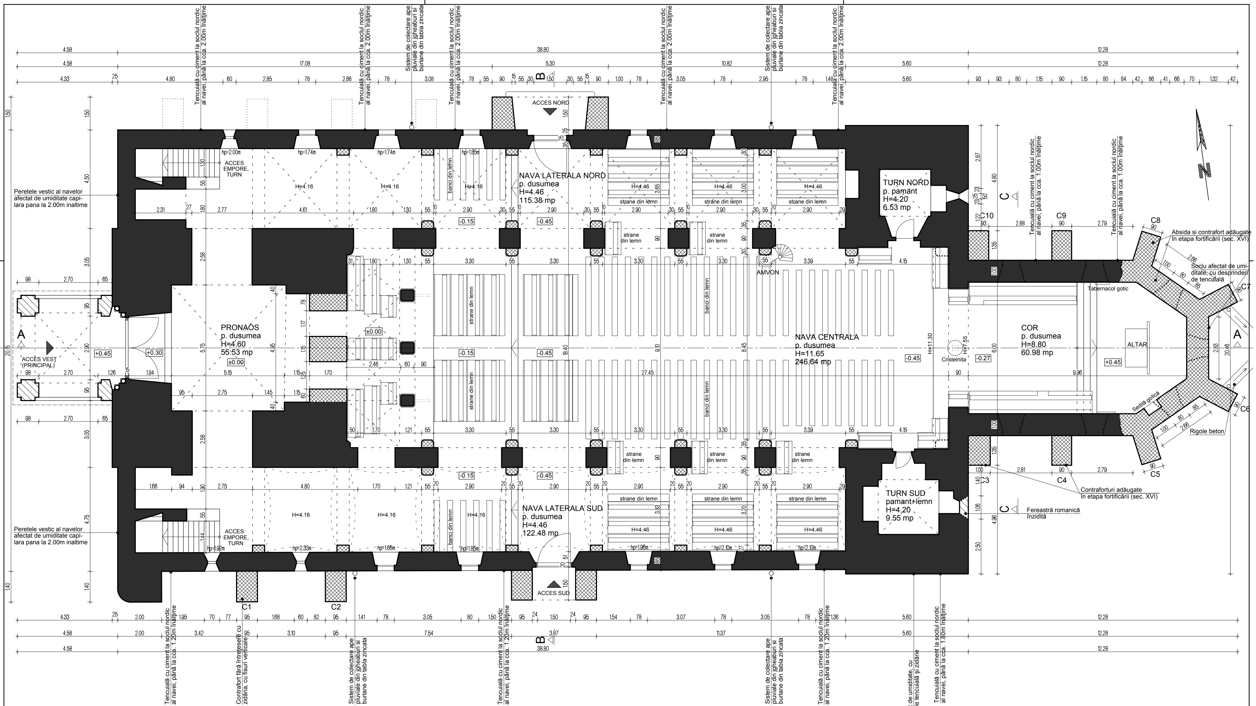
RELEVU BISERICA - PLAN PARTER (COTA +2.50) scara 1:100
