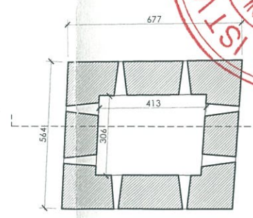
PLAN COTA +11.00 m
