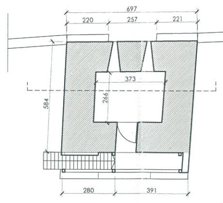
PLAN COTA +5.80 m
