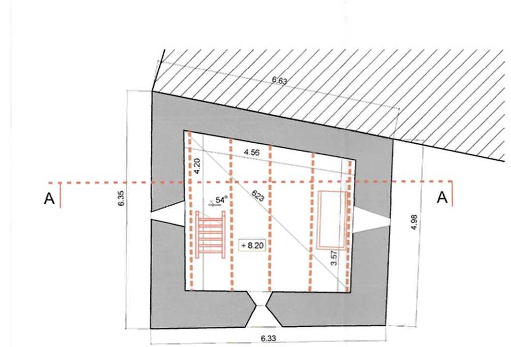
PLAN COTA +9.40 m
