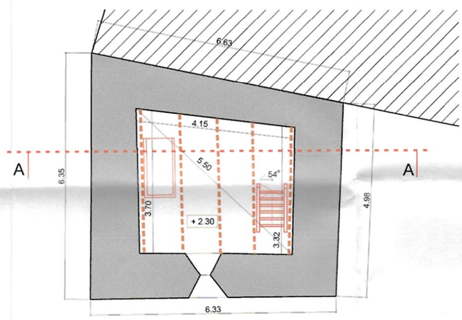
PLAN COTA +3.00 m
