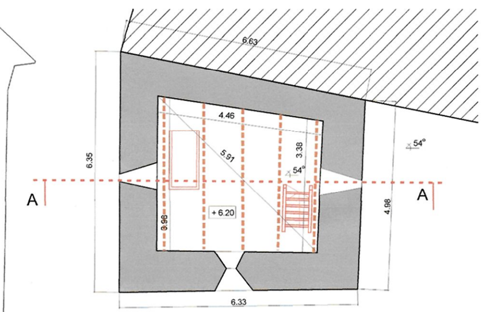
PLAN COTA +7.20 m
