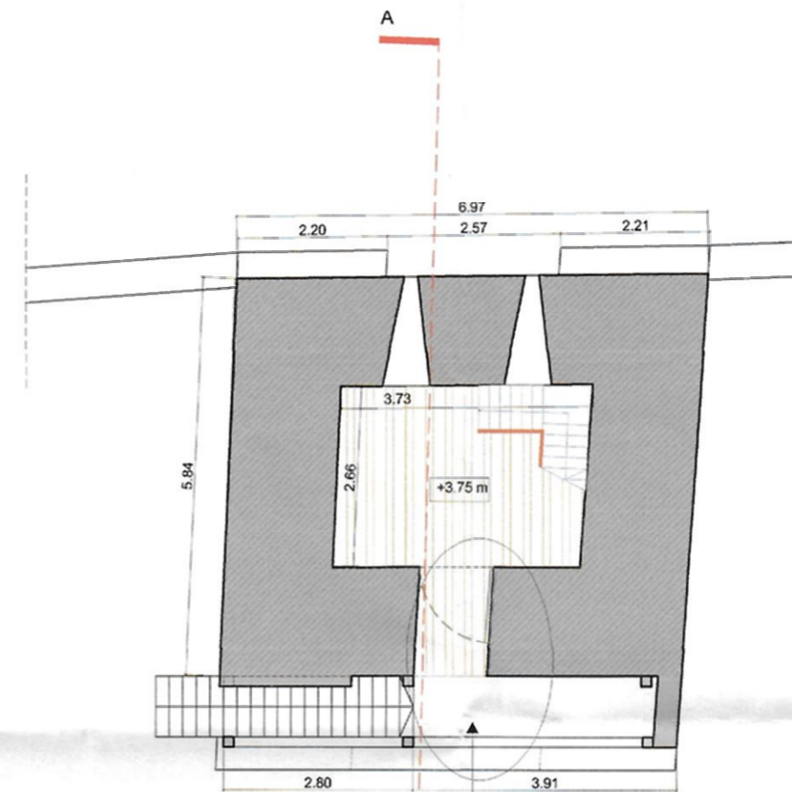
PLAN COTA +5.80 m
