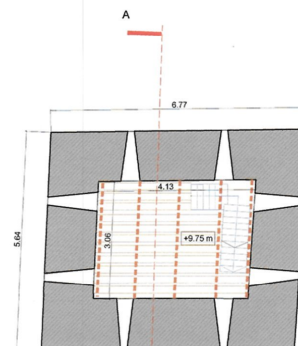
PLAN COTA +11.0 m
